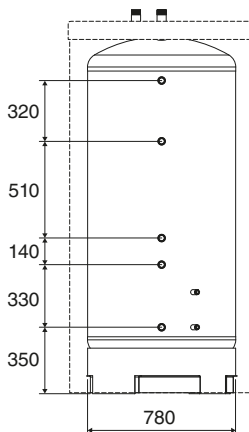
Smart ME 800
